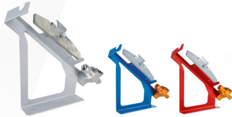
TP165-ARROW FLETCHING JIG
